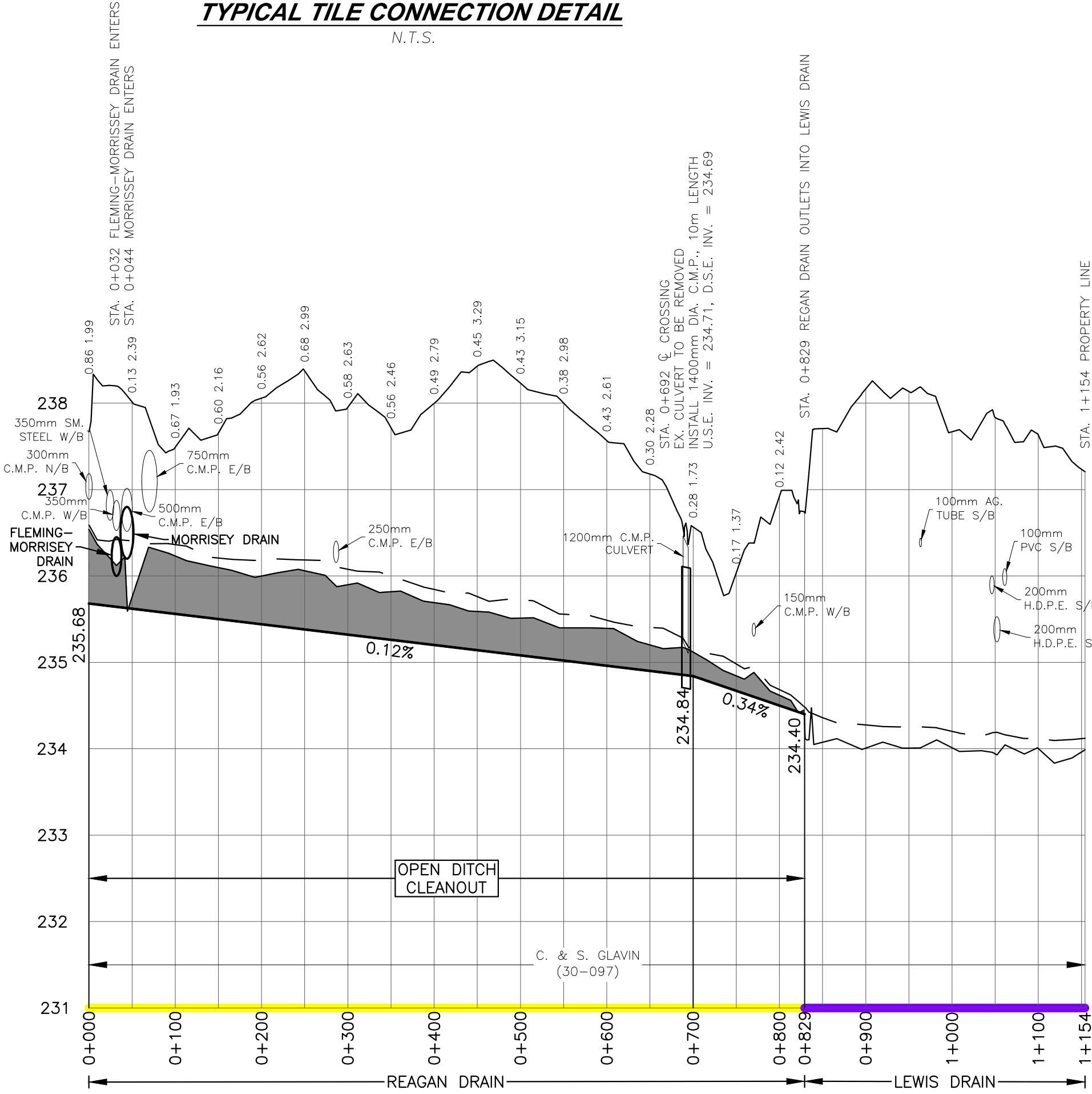
REGAN DRAIN PROFILE
