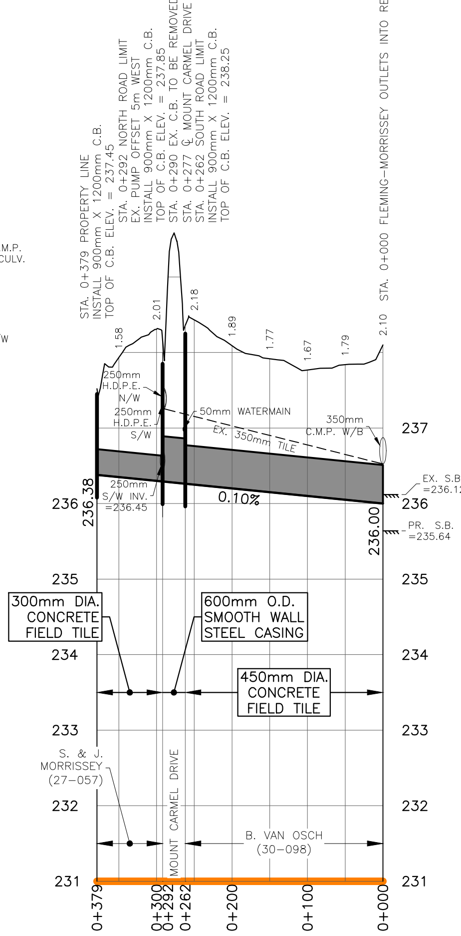
FLEMING-MORRISSEY DRAIN PROFILE
