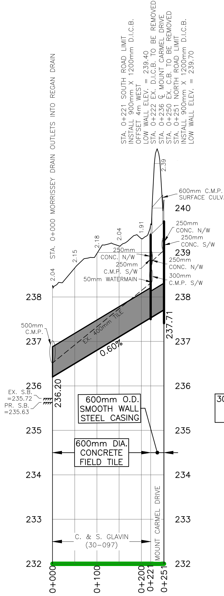
MORRISSEY DRAIN PROFILE
