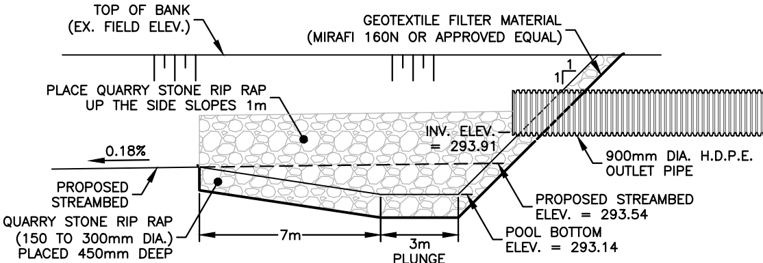
PLUNGE POOL DETAIL
