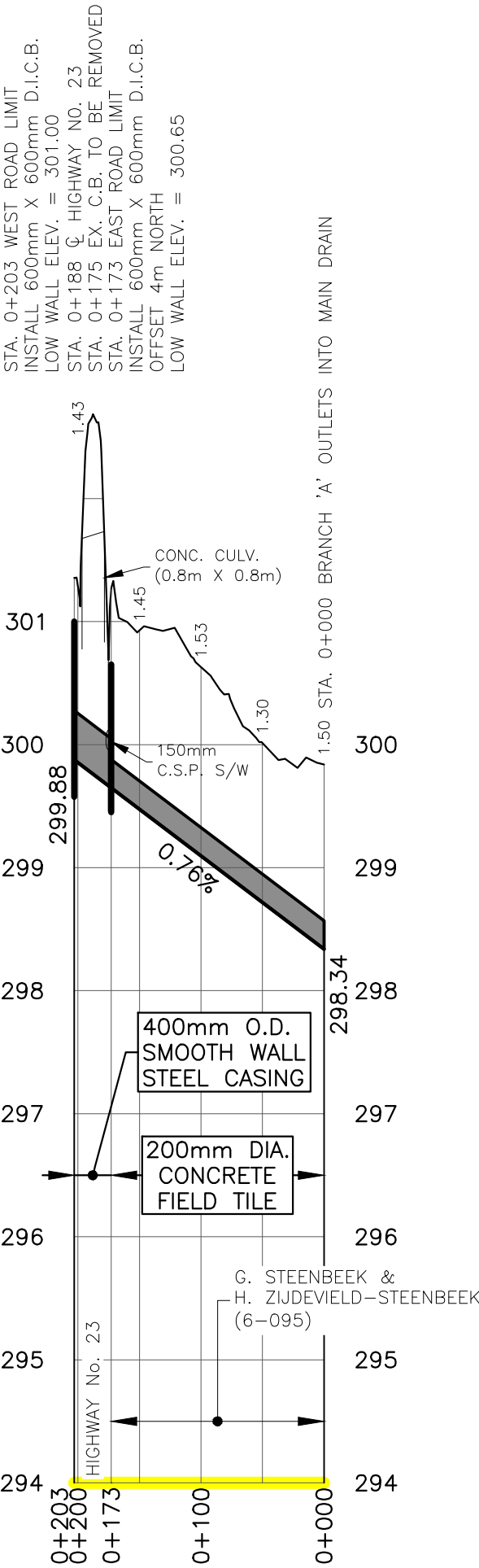
BRANCH 'A' PROFILE
