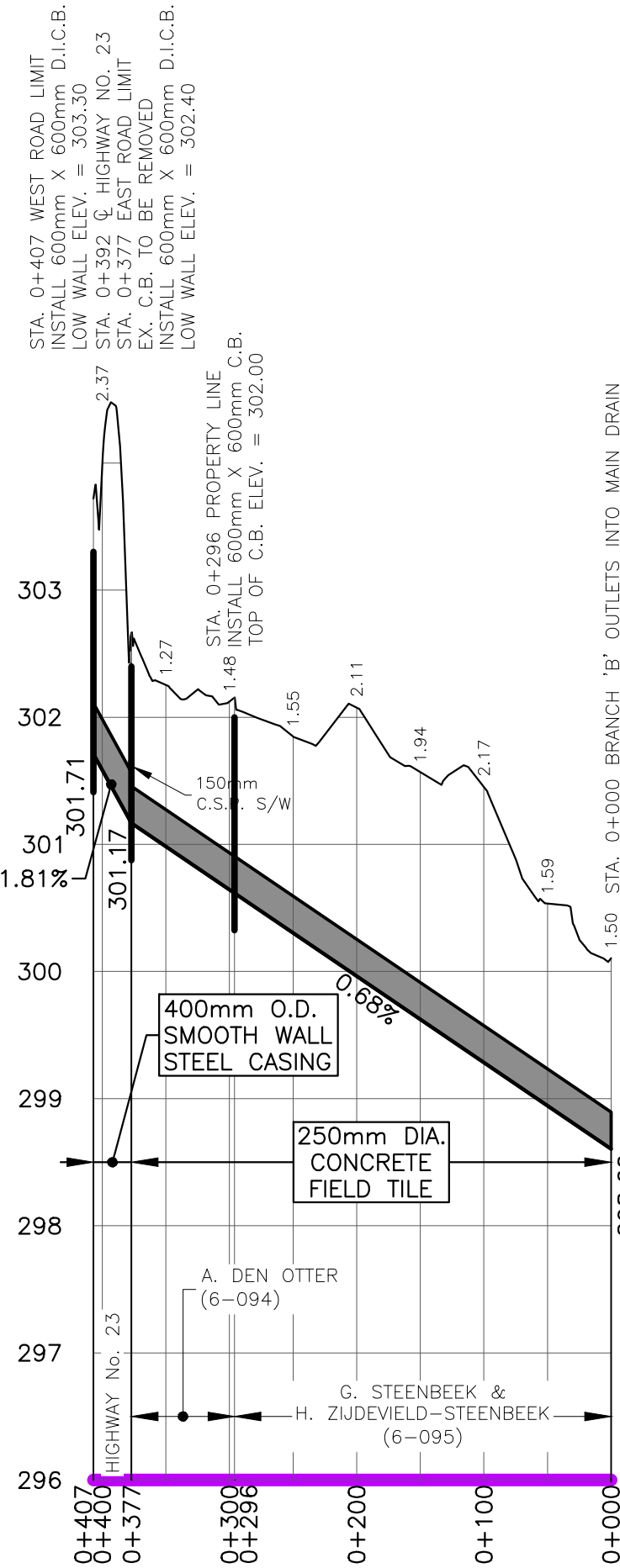
BRANCH 'B' PROFILE
