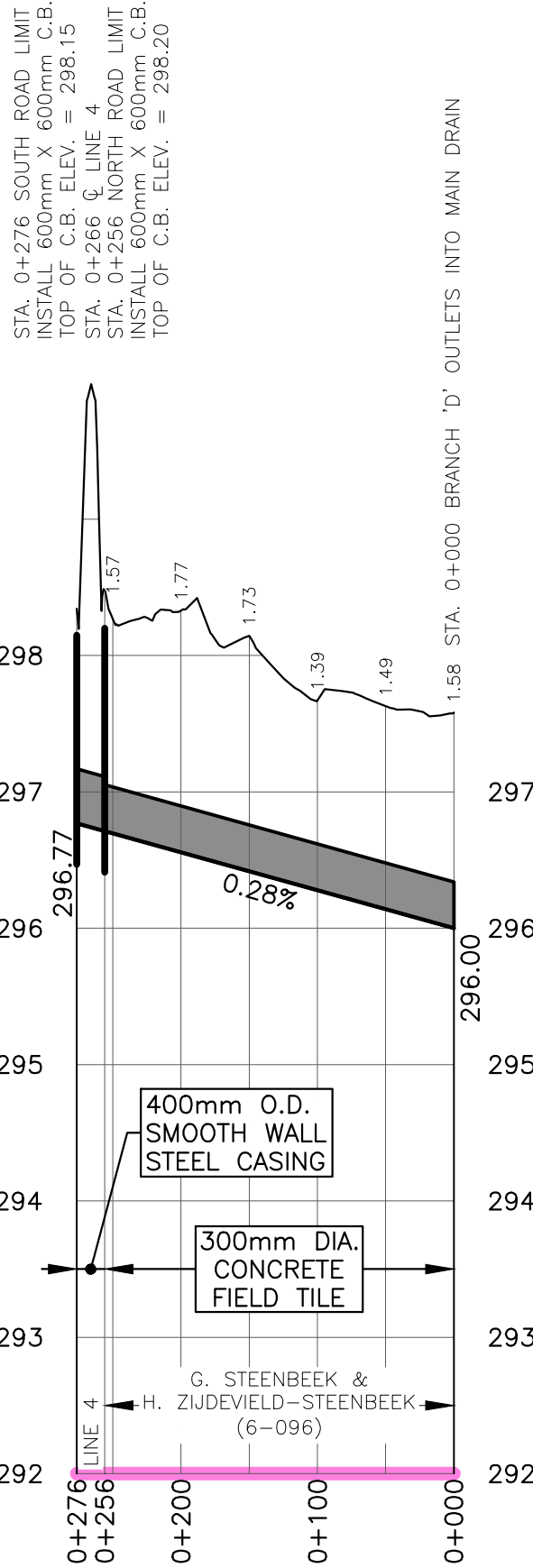
BRANCH 'D' PROFILE
