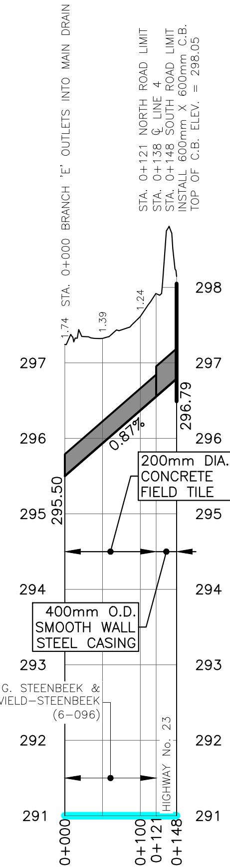
BRANCH 'E' PROFILE
